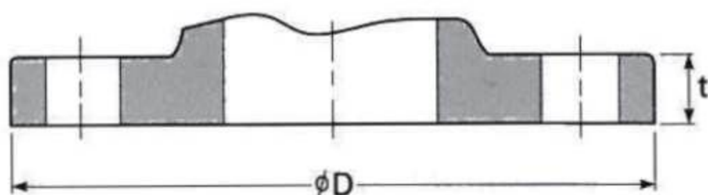
Full face(FF)
