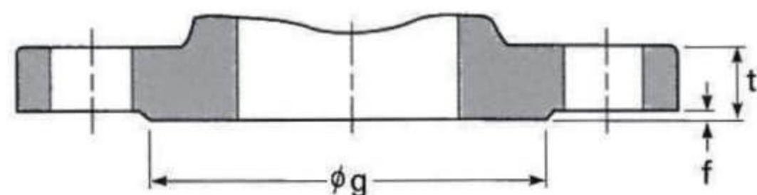
Raised face(RF)
