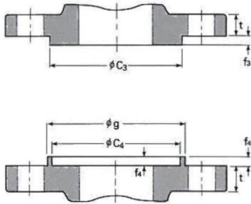
Male-female face(MF)
