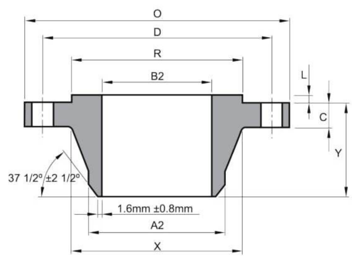
WELDING NECK
