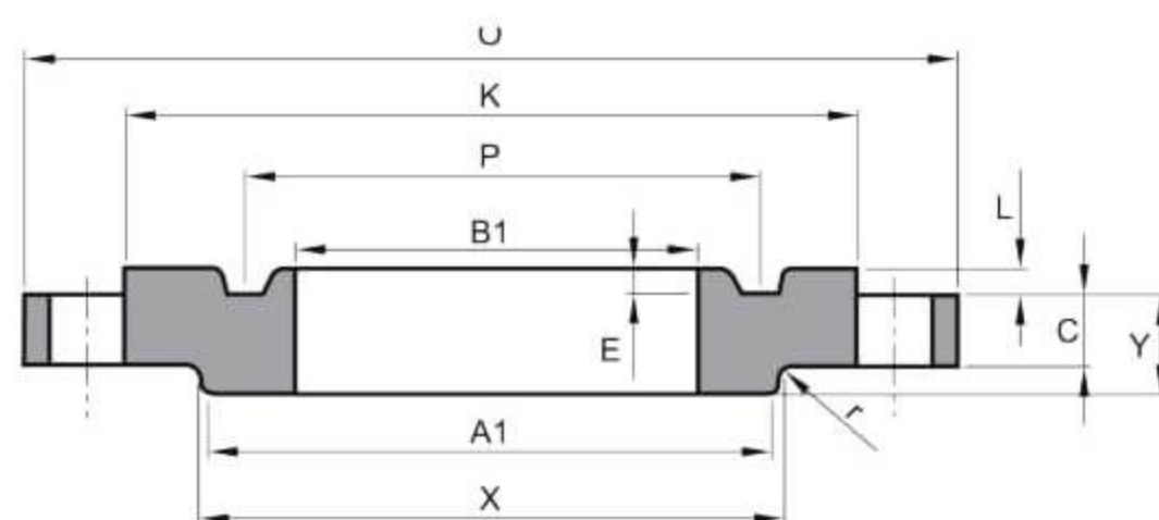
SLIP-ON RING JOINT
