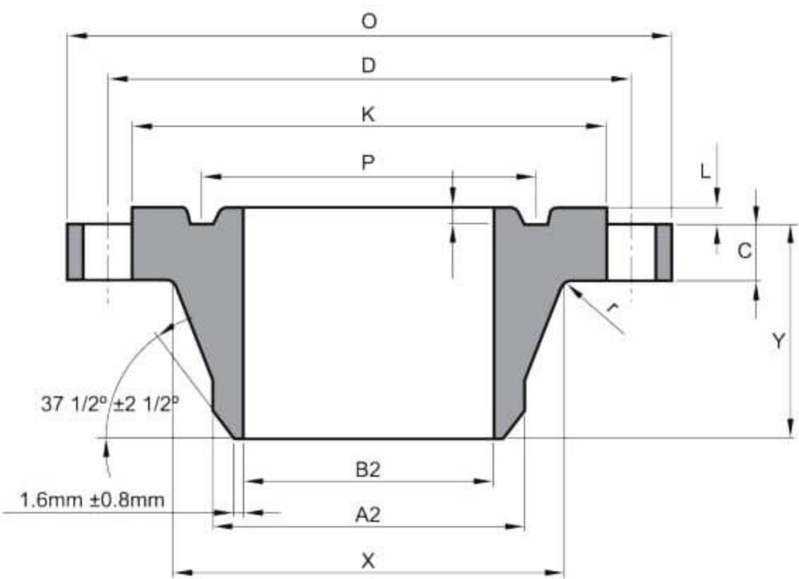
WELDING NECK RING JOINT
