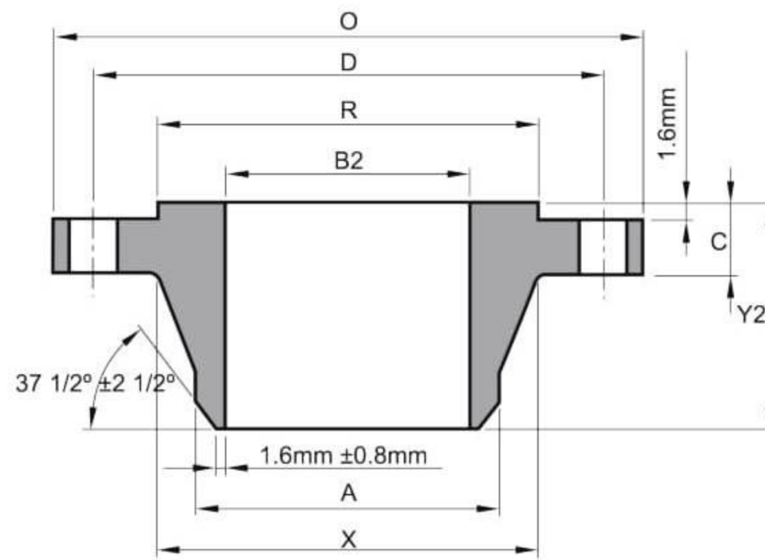
WELDING NECK
