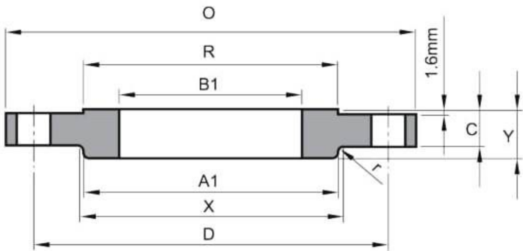
SLIP-ON
