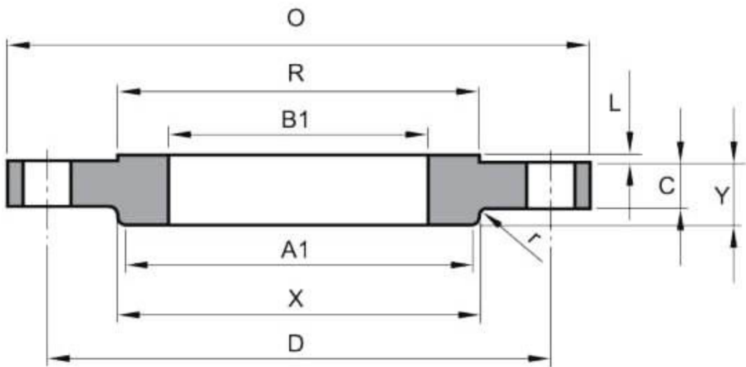
SLIP-ON
