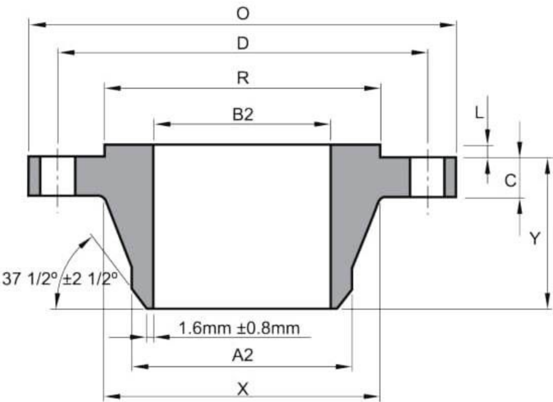
WELDING NECK
