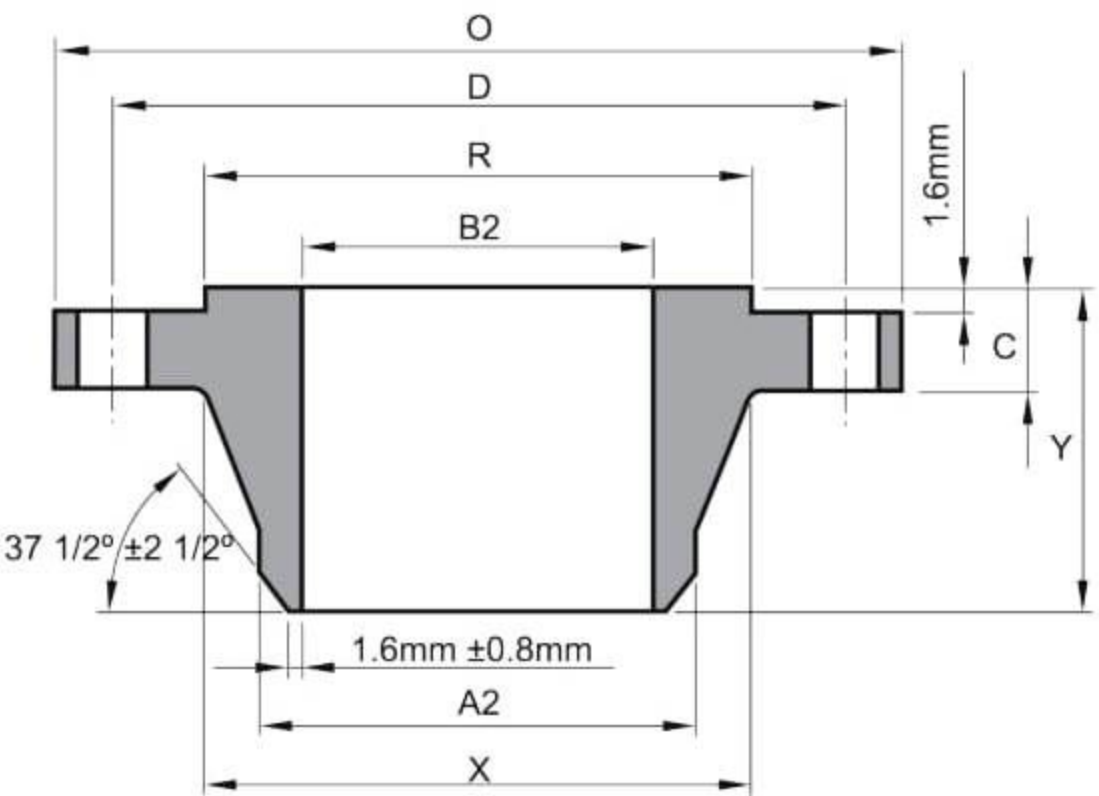
WELDING NECK
