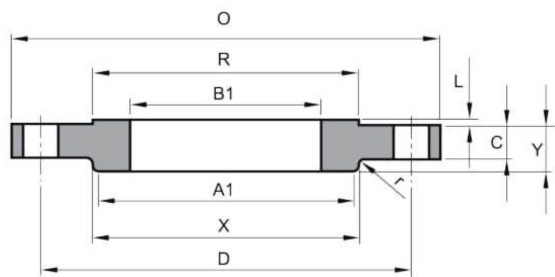
SLIP-ON
