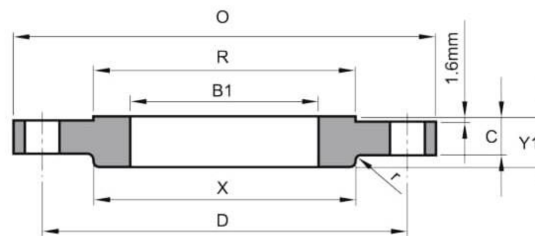
SLIP-ON
