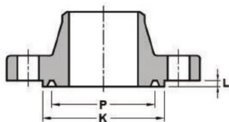
WELDING NECK
