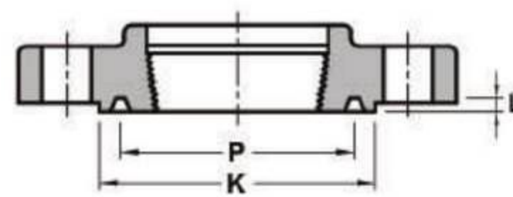
THREADED
