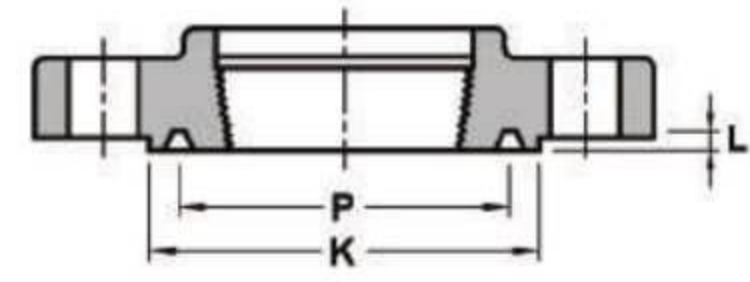
THREADED
