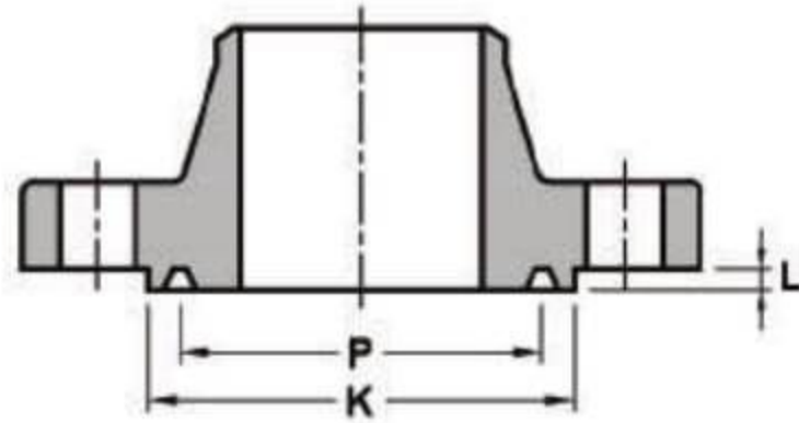
WELDING NECK
