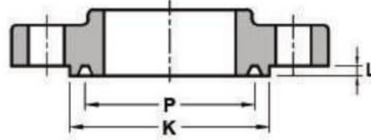
SLIP-ON
