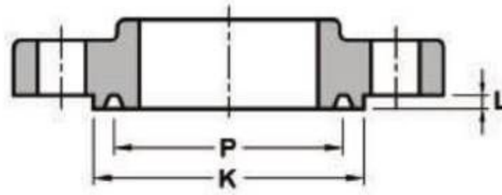
SLIP-ON
