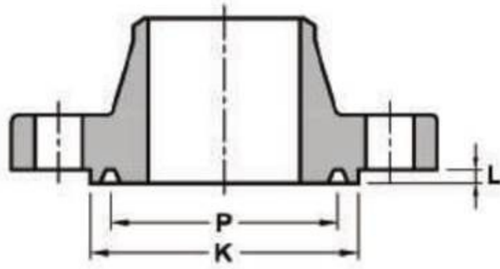
WELDING NECK
