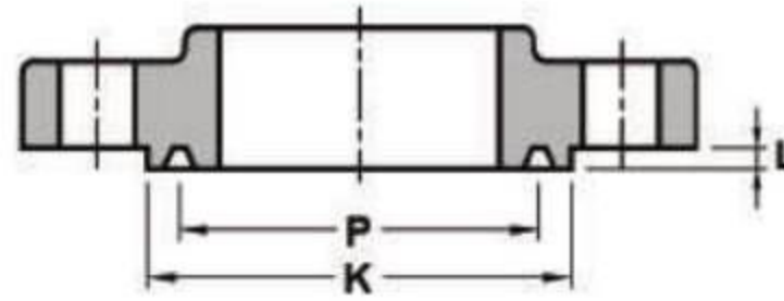
SLIP-ON
