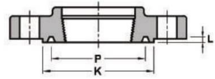
THREADED
