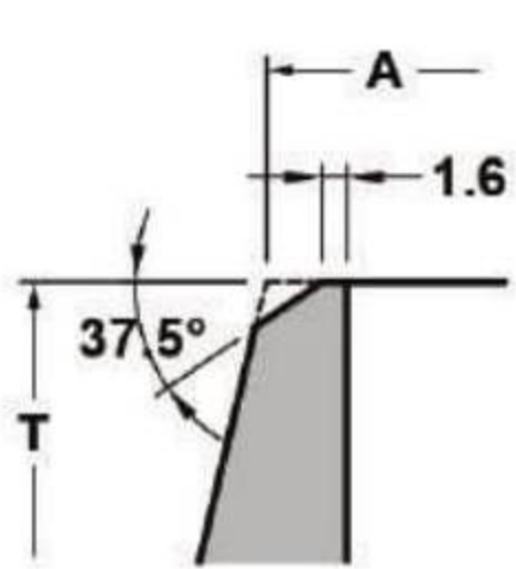
Detail "w" Typical Welding end Prepration
