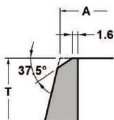
Detail "w" Typical Welding end Preparation
