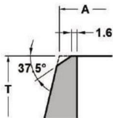
Detail "w" Typical Welding end Prepration
