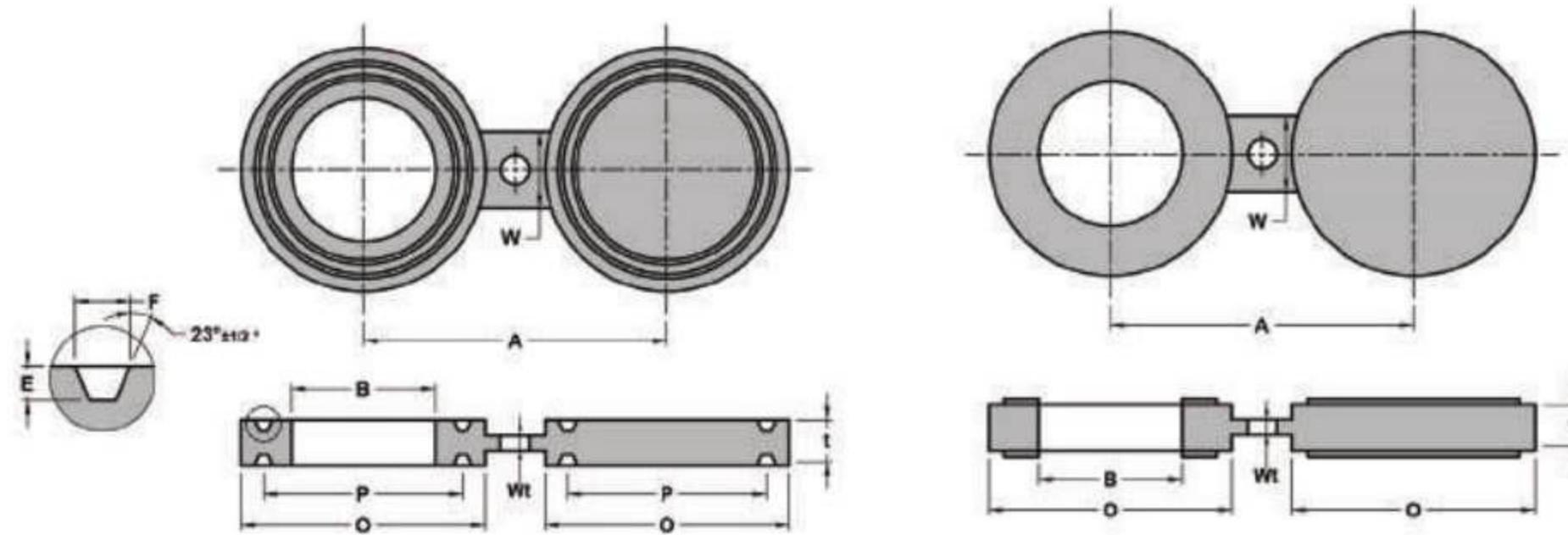
Class 600 FIGURE 8 BLANK RAISED FACE & FEMALE RING-JOINT FACING
