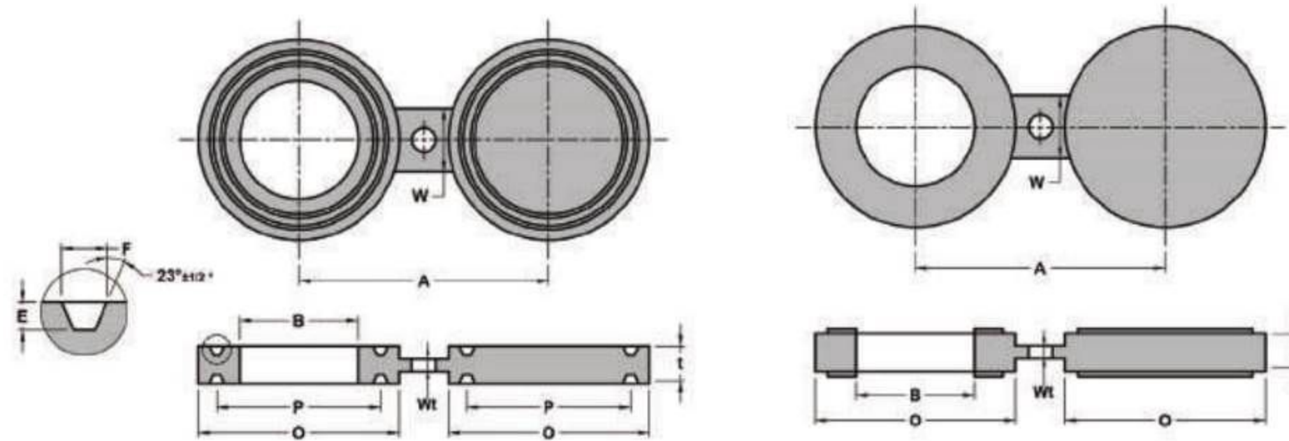
Class 150 FIGURE 8 BLANK RAISED FACE & FEMALE RING-JOINT FACING
