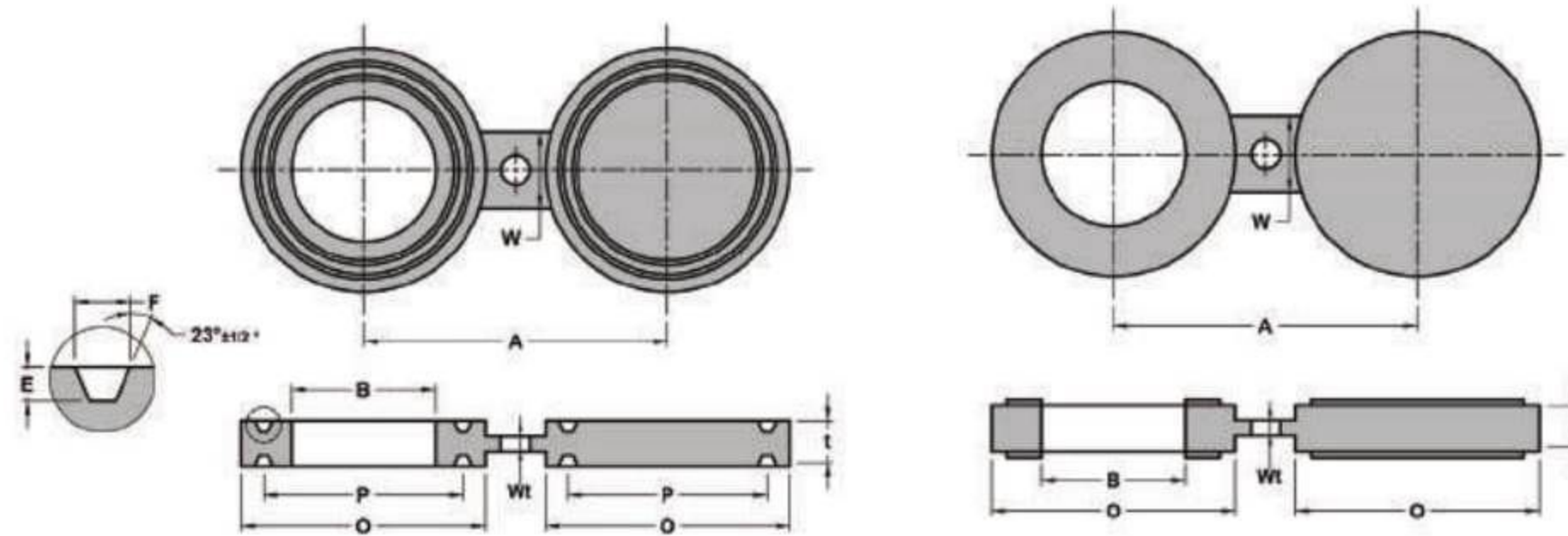
Class 1500 FIGURE 8 BLANK RAISED FACE & FEMALE RING-JOINT FACING
