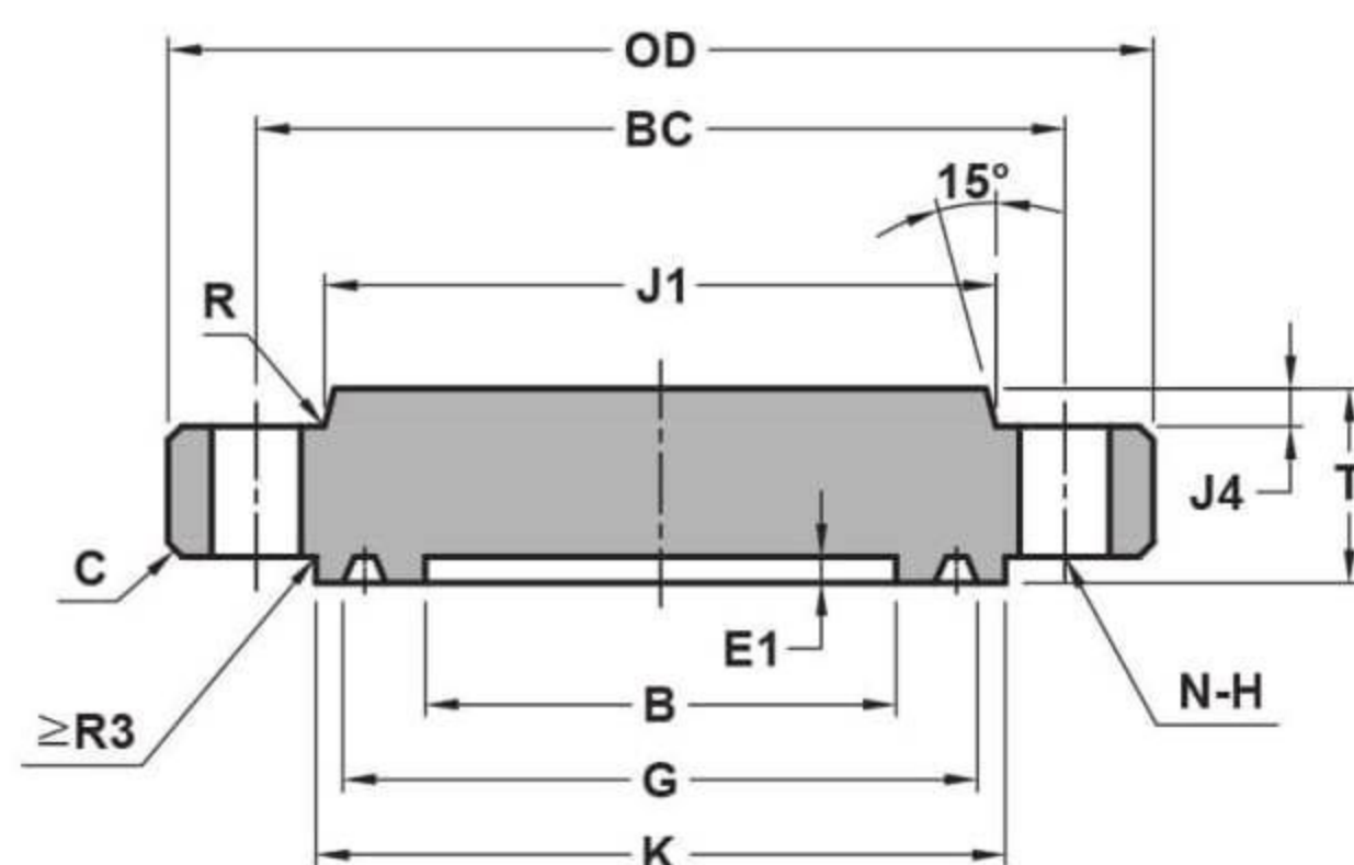
BLIND RTJ
