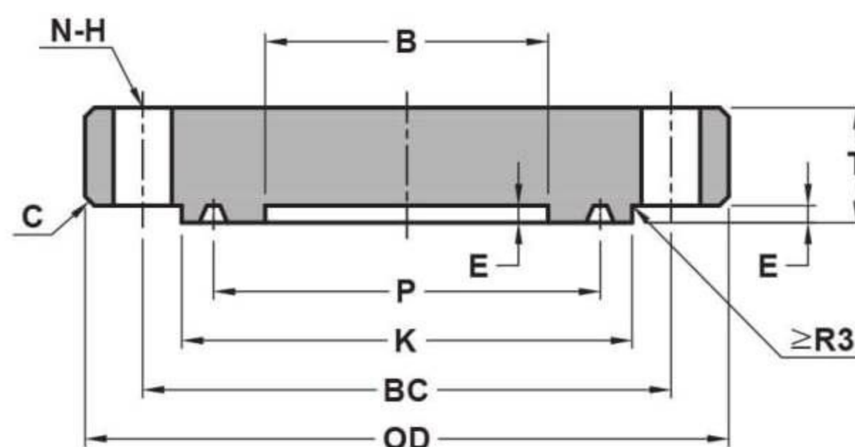
BLIND RTJ
