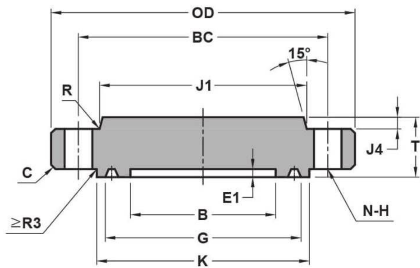
BLIND RTJ
