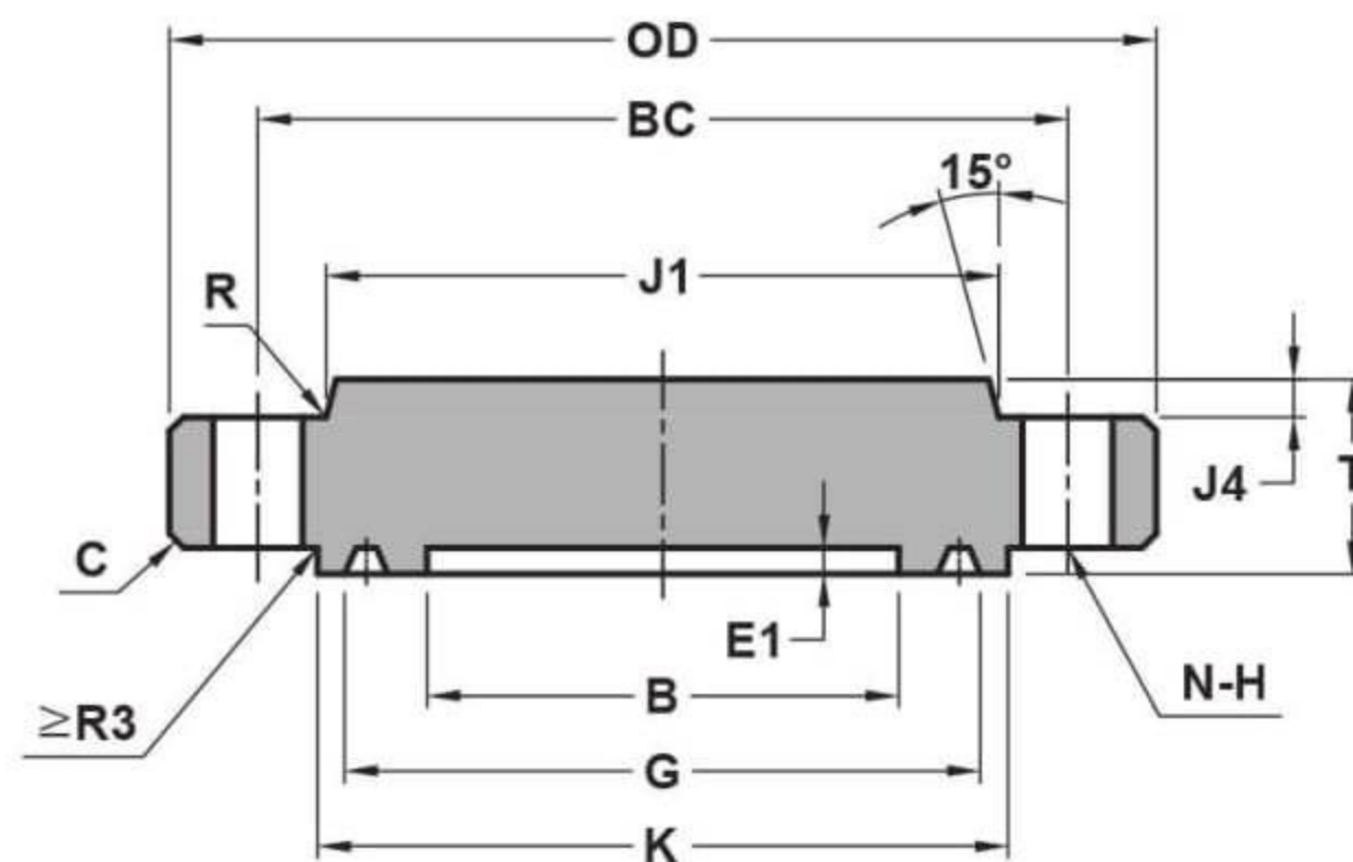
BLIND RTJ
