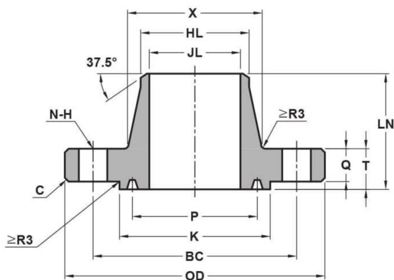
WELDING NECK RTJ
