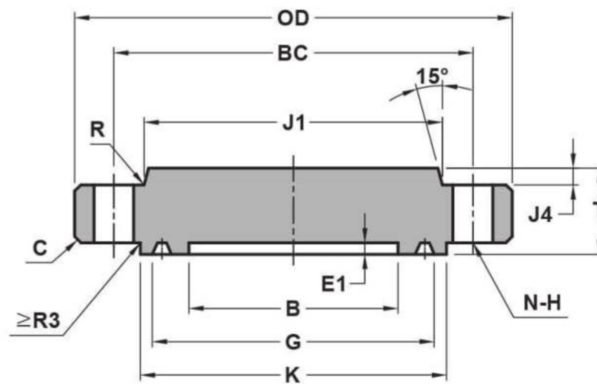
BLIND RTJ
