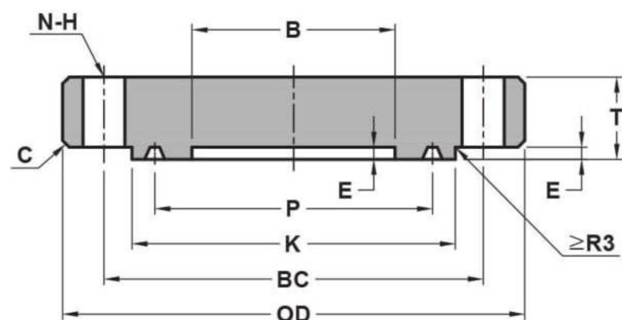
BLIND RTJ
