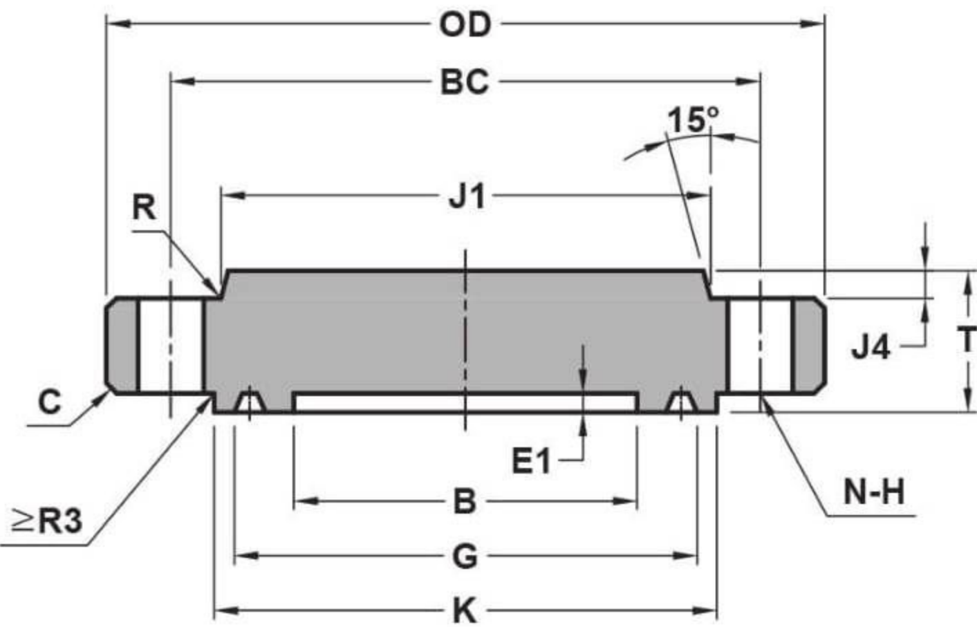
BLIND RTJ
