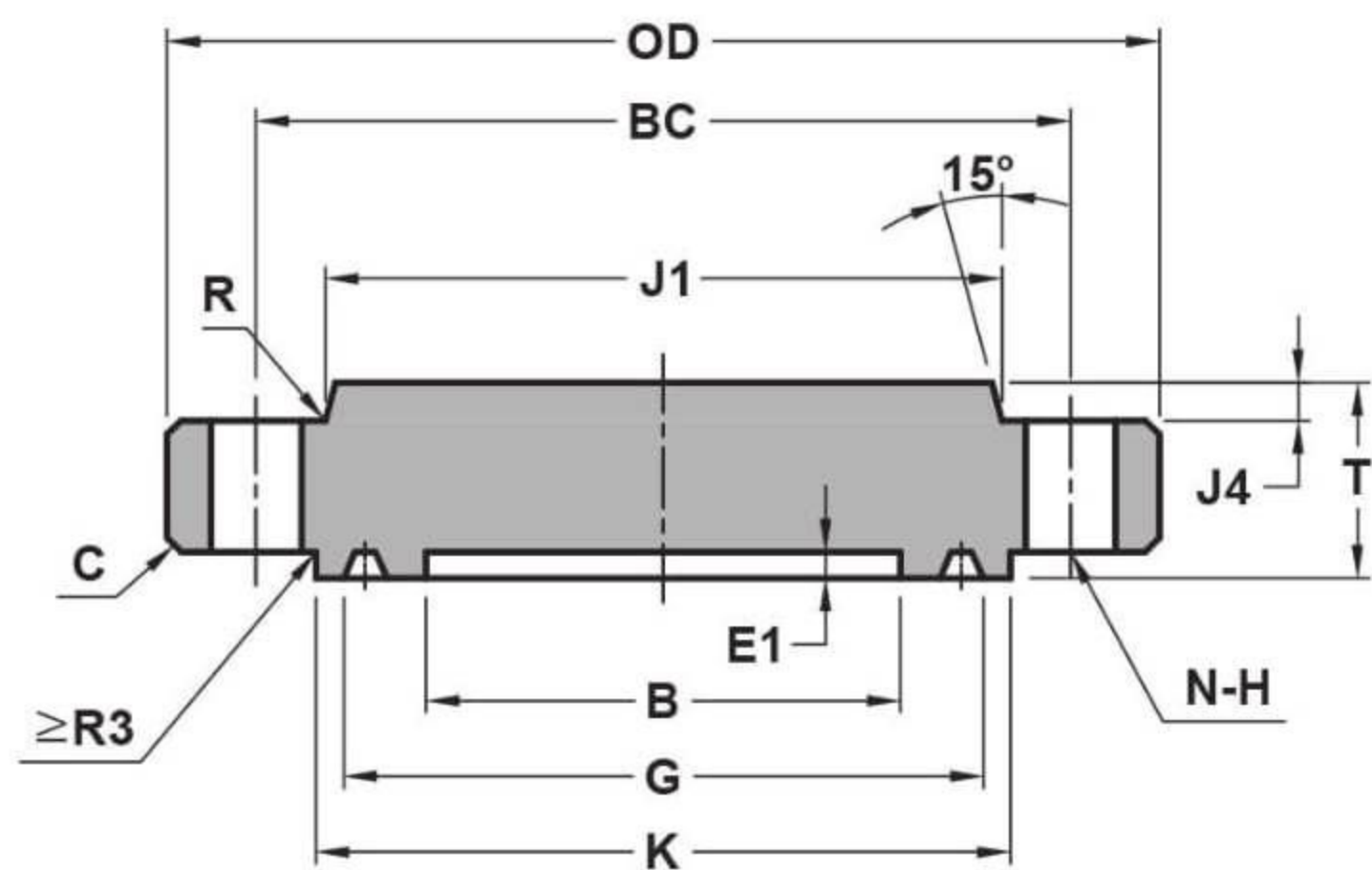
BLIND RTJ
