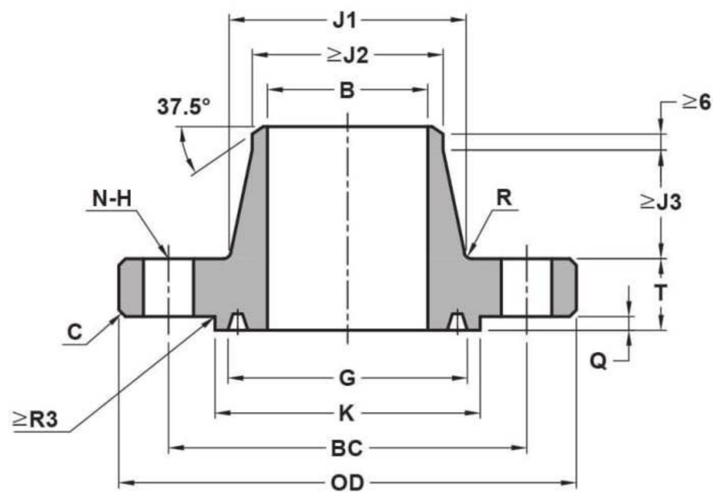
WELDING NECK RTJ
